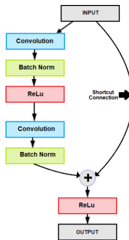
Figure 4: Residual Learning: A building block
