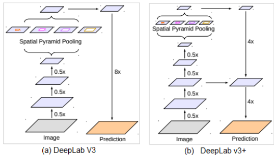
Figure 11: DeepLabV3 and DeepLabV3+ [101]
